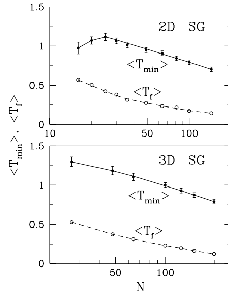
Figure 10. The same as in figure 8 but for the DFM systems. Figure 11. The same as in figure 8 but for the SG systems.
