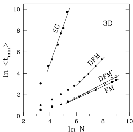
Figure 4. Scaling of t_{\text{min}} for 3D FM, DFM', DFM and SG.
