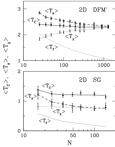
Figure 12. The size dependence of T_C , T_\chi , T_s and T_f for the 2D DFM' and SG systems.
