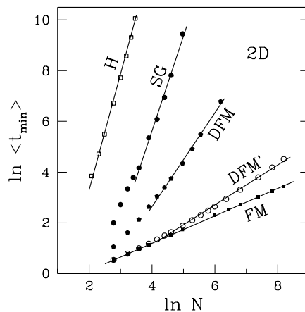
Figure 3. The scaling of t_{\text{min}} for 2D FM, DFM', DFM, SG and the 'helices'.
