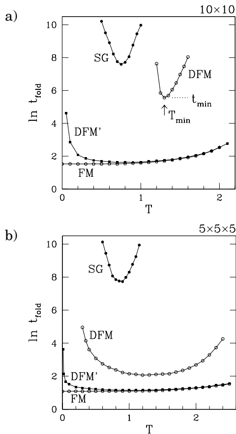
Figure 1. The temperature dependence of the characteristic 'folding' time for the (a) 2D and (b) 3D FM, DFM', DFM and SG Ising systems. Here, L = 10 for the 2D, and 5 for the 3D systems. The number of starting configurations is equal to 1000.
