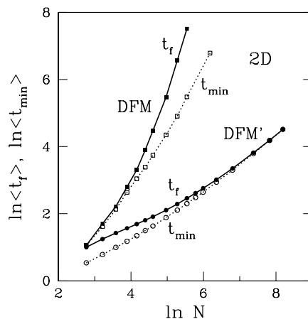
Figure 5. Scaling of t_f for 2D DFM and DFM' (solid curves) compared to the scaling of t_{\text{min}} (dotted curves). The effective slope for the last three data points corresponding to DFM is 3.54.
