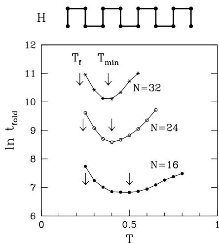
Figure 2. The top of the figure shows an example of a 'helical' conformation on the 2D lattice used in this paper. The conformation shown is for N = 16 . The lower part shows the dependence of t_{\text{fold}} on T for three indicated lengths of the 'helix'. The values of T_f and T_{\text{min}} are marked by the arrows.
