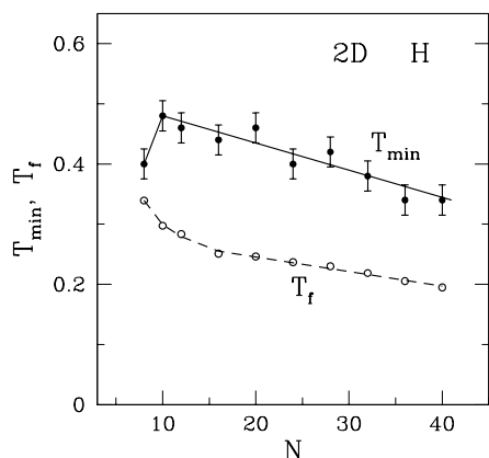
Figure 7. The same as in figure 6 but for 2D Go models of the 'helices'.
