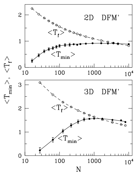
Figure 9. The same as in figure 8 but for the DFM' systems.
