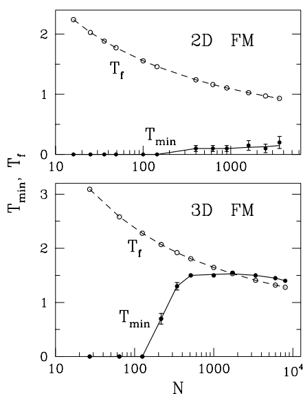
Figure 8. The dependence of T_f and T_{\min} of 2D and 3D FM on N .
