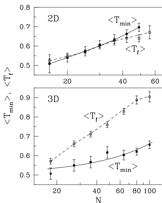
Figure 6. Scaling of T_f and T_{\min} for the 2D and 3D lattice Go models of proteins. Data points are taken from [2].
